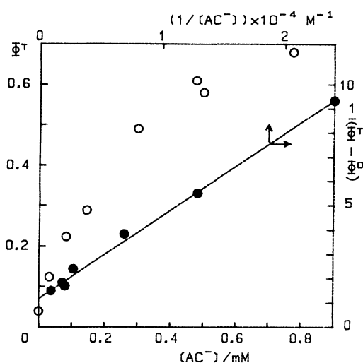
Fig. 2. AC^- concentration effect on the quantum yield of MV^+ formation through the energy transfer from ^3Ery^{2-} to AC^- , \Phi^T . [ Ery^{2-} ]: 5 \mu M ; [ MV^{2+} ]: 0.1 mM ; [TEOA]: 3 mM ; pH=8.5 ; \mu=0.1 .
